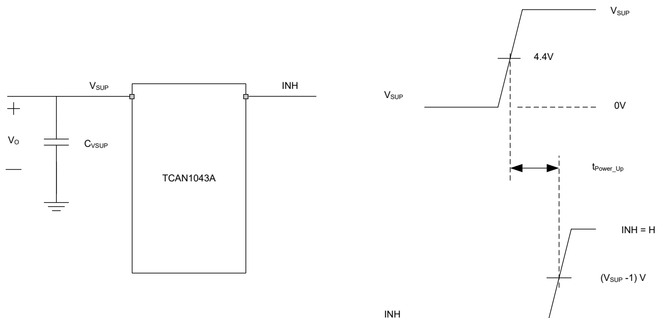
图 7-10. Power-Up Timing
