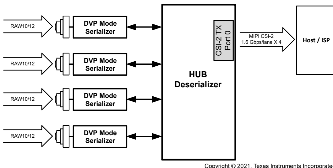
图 8-14. Four DVP Mode Serializers Sensor Data Onto CSI-2 Over 1 Port
