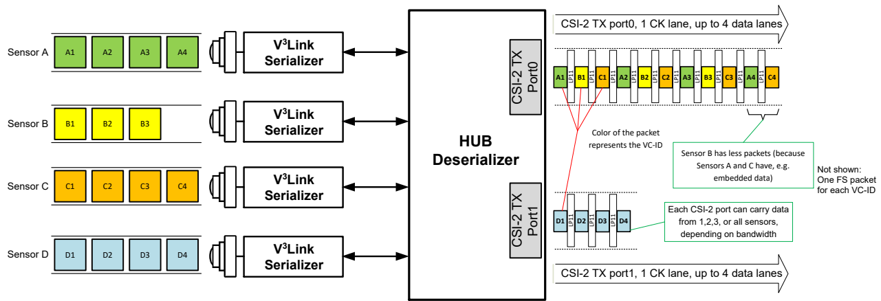
图 7-13. Four Sensor Data onto CSI-2 With Virtual Channels (VC-ID) With Different Frame Size
