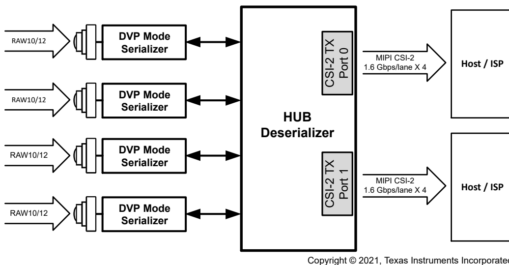
图 8-15. Four DVP Mode Serializers Sensor Data Onto CSI-2 Over 2 Ports
