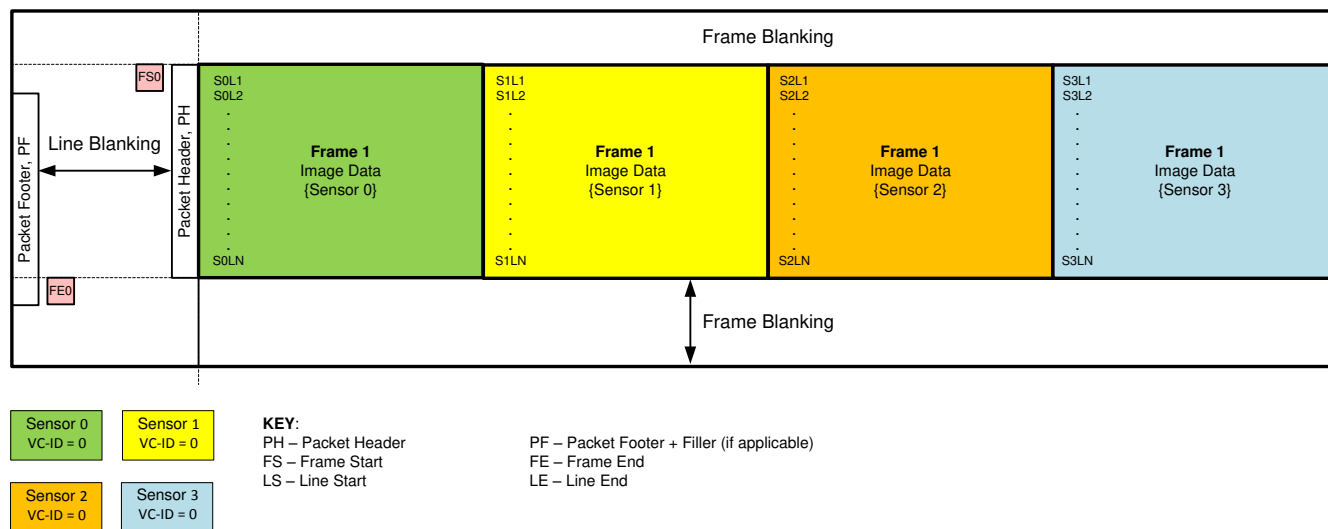
图 7-20. Line-Concatenated Format
