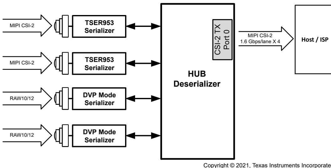
图 8-16. Two DVP Mode Serializers and Two TSER953 Sensor Data Onto CSI-2 Over 1 Port
