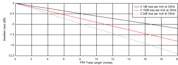
图 9-3. FR4 Trace Insertion Loss at 3 GHz
