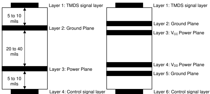
图 9-10. Recommended 4 or 6-Layer PCB Stack
