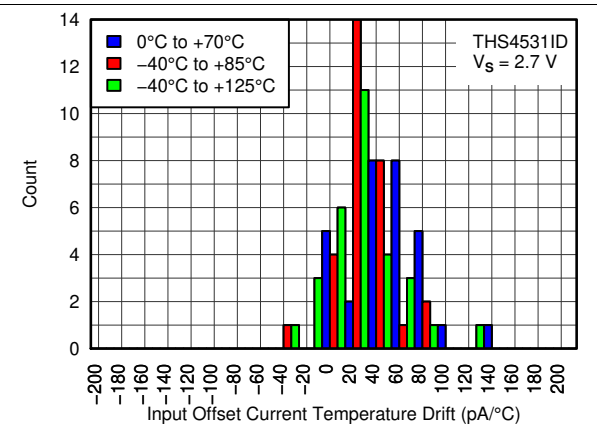
Figure 30. Input Offset Current Temperature Drift Histogram
