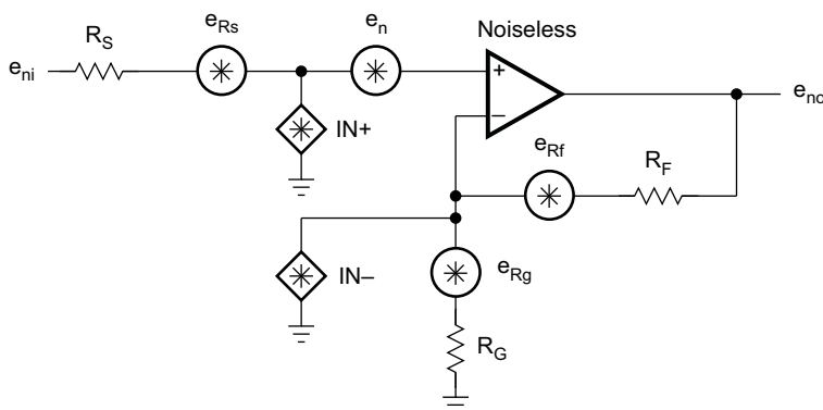
Figure 51. Noise Model
