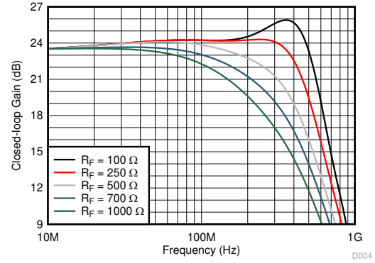
图 5-6. Small-Signal Frequency Response vs R_F
