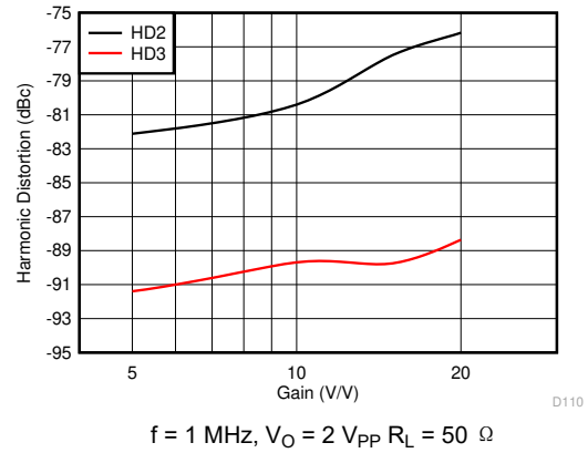
图 5-44. Harmonic Distortion vs Gain
