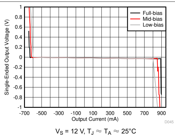
图 6-4. Linear Single-Ended Output Voltage vs I_O and Temperature
