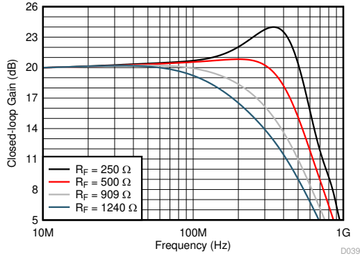
图 5-5. Small-Signal Frequency Response vs R_F
