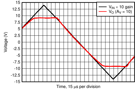
图 5-24. Overdrive Recovery
