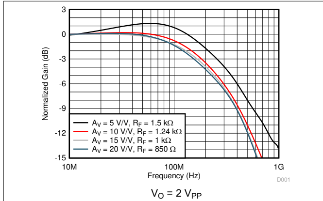
图 5-1. Small-Signal Frequency Response
