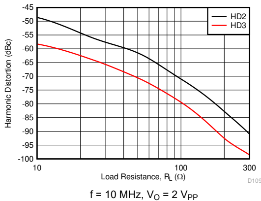
图 5-48. Harmonic Distortion vs R_L
