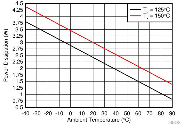
图 6-2. Package Power Dissipation vs Ambient Temperature
