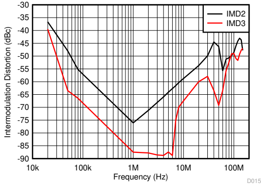
图 5-23. Intermodulation Distortion vs Frequency
