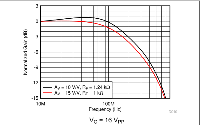
图 5-2. Large-Signal Frequency Response
