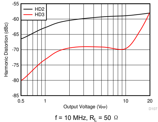
图 5-46. Harmonic Distortion vs V_O
