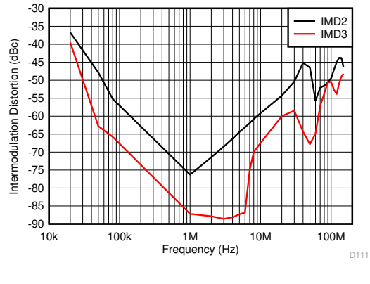
图 5-42. Intermodulation Distortion vs Frequency
