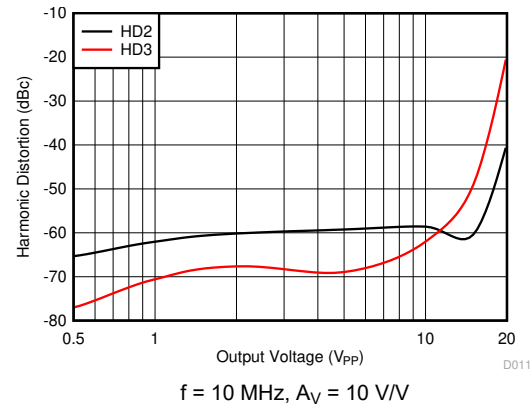
图 5-20. Harmonic Distortion vs V_O
