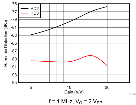
图 5-18. Harmonic Distortion vs Gain
