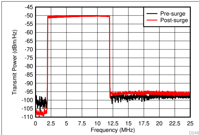
图 6-8. China SGCC HPLC Band0 Pre-Surge and Post-Surge
