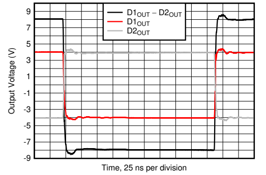
图 5-24. Overdrive Recovery
