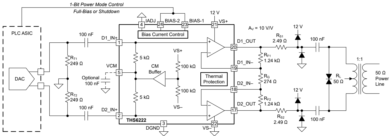
图 7-1. Typical Broadband PLC Configuration
