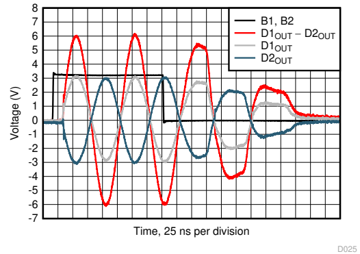
图 5-36. Full-Bias and Shutdown Mode Transition Timing
