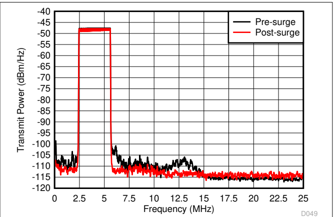
图 6-9. China SGCC HPLC Band1 Pre-Surge and Post-Surge
