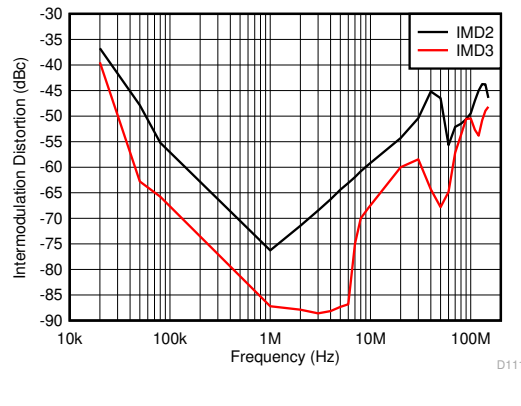
图 5-42. Intermodulation Distortion vs Frequency
