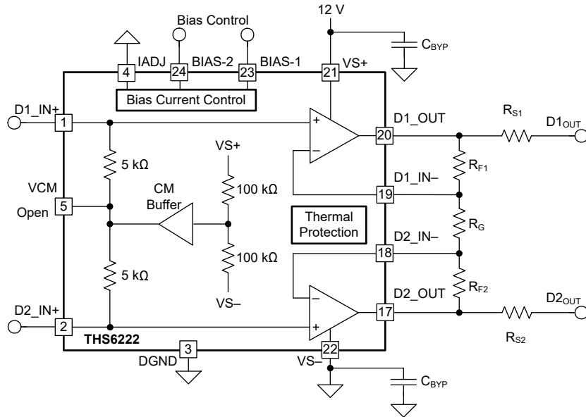
图 7-5. Representative Schematic for the Layout in 图 7-6
