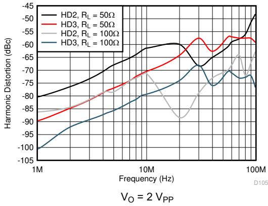
图 5-43. Harmonic Distortion vs Frequency
