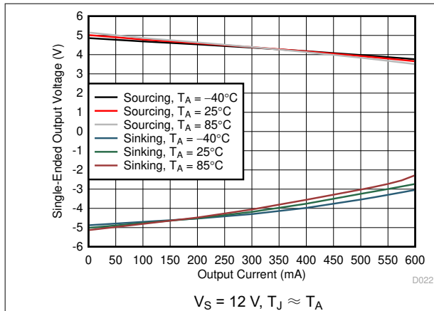
图 6-3. Slammed Single-Ended Output Voltage vs I_O and Temperature
