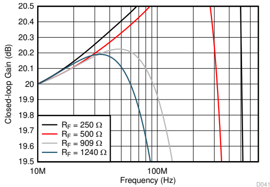
图 5-5. Small-Signal Frequency Response vs R_F
