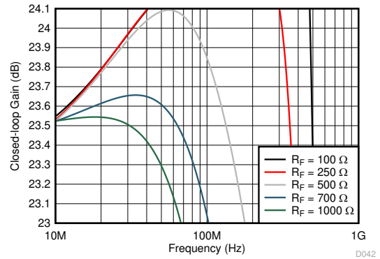
图 5-6. Small-Signal Frequency Response vs R_F
