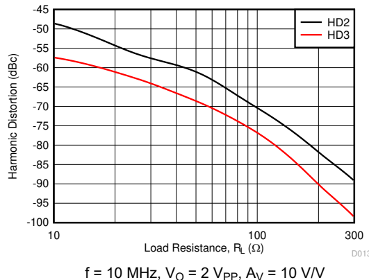
图 5-22. Harmonic Distortion vs R_L
