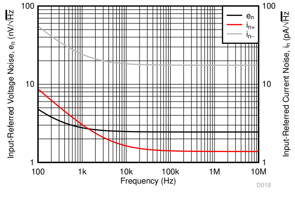
图 5-16. Input Voltage and Current Noise Density vs Frequency
