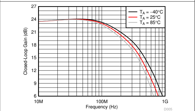
图 5-2. Large-Signal Frequency Response
