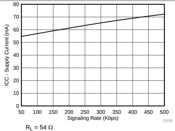
图 8. THVD1510 Supply Current vs Signal Rate
