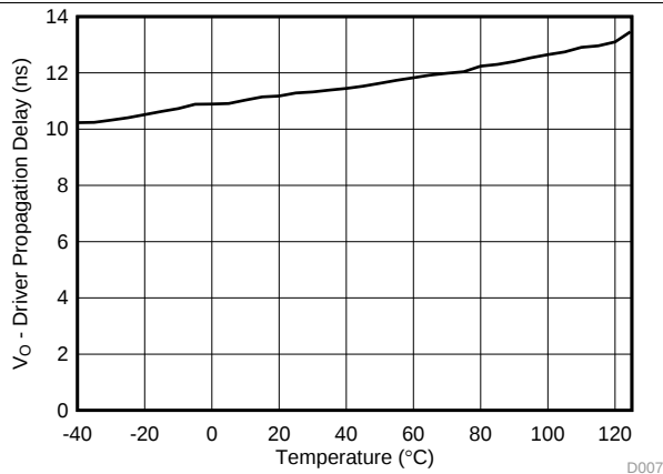
图 7. THVD1550 Driver Propagation Delay vs Temperature
