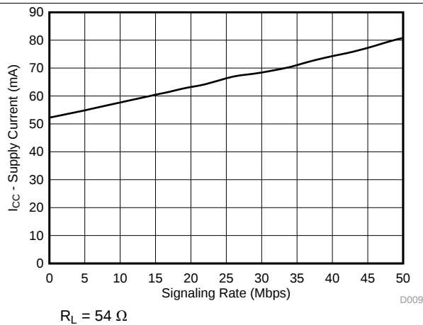
图 9. THVD1550 Supply Current vs Signal Rate
