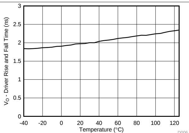
图 4. THVD1510 Driver Rise or Fall Time vs Temperature
