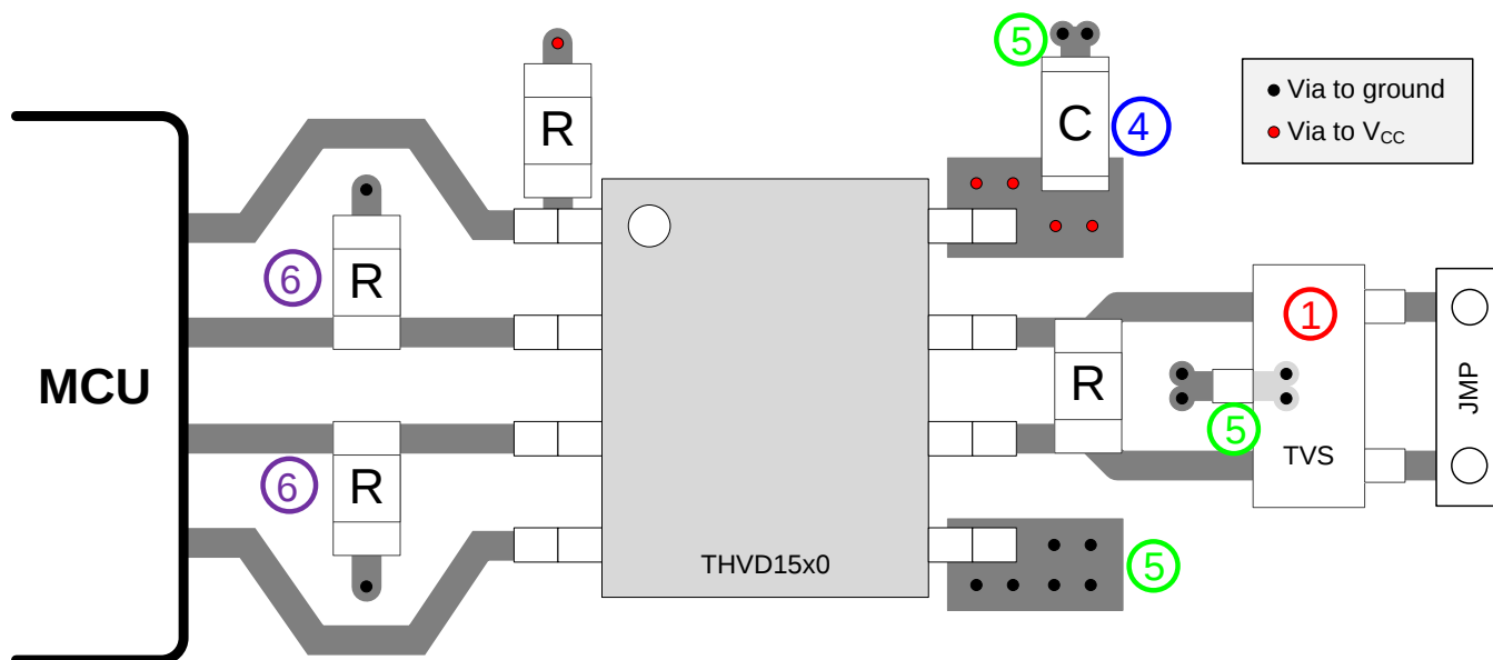
图 32. Half-Duplex Layout Example
