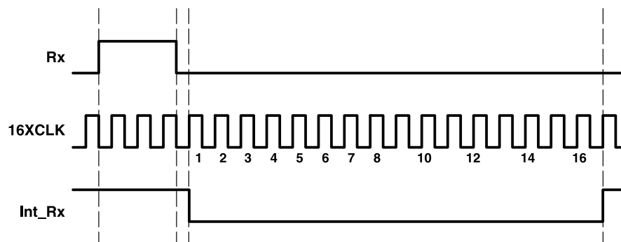
Figure 33. Positive Rx Pulse Decode – Detailed View
