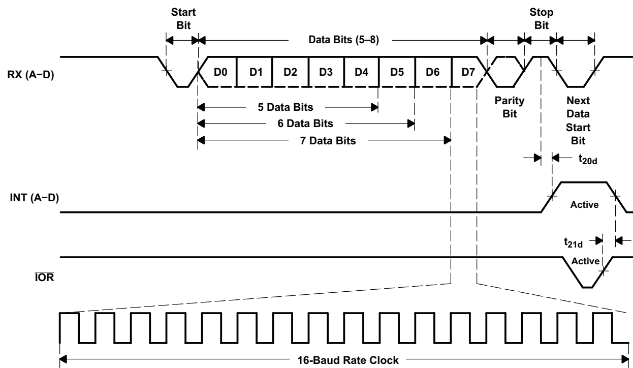
Figure 16. Receive Timing
