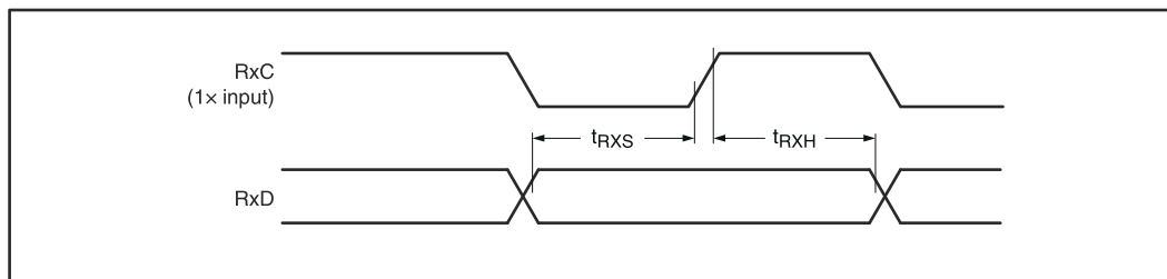
图 4-11. Receiver External Clocks
