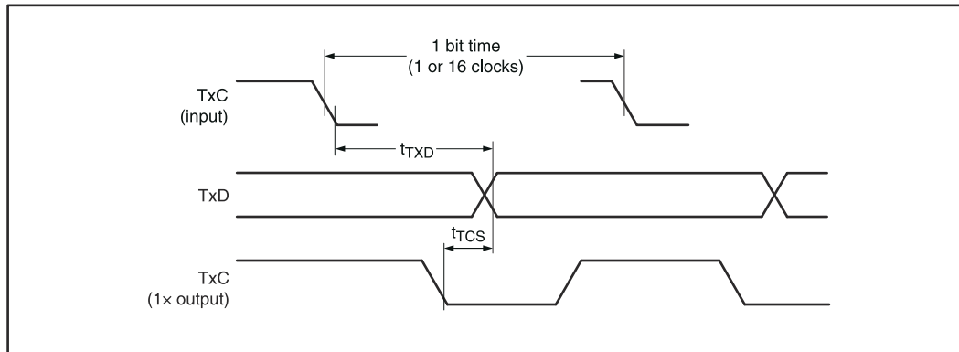
图 4-10. Transmitter External Clocks
