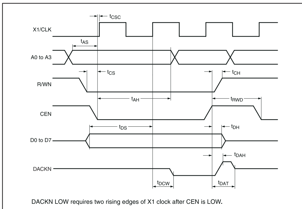
图 4-5. Bus Timing, Write Cycle (68xxx Mode)
