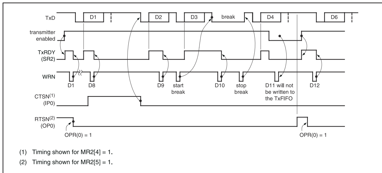
图 4-12. Transmitter Timing
