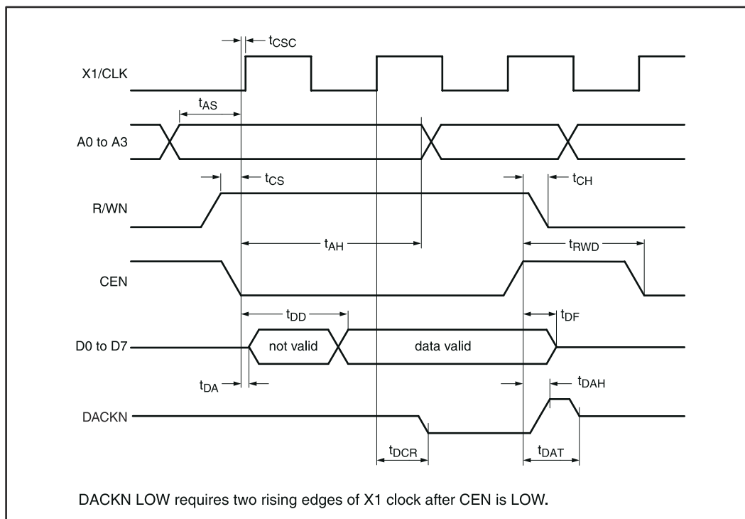
图 4-4. Bus Timing, Read Cycle (68xxx Mode)
