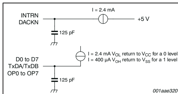
图 4-14. Test Conditions on Outputs
