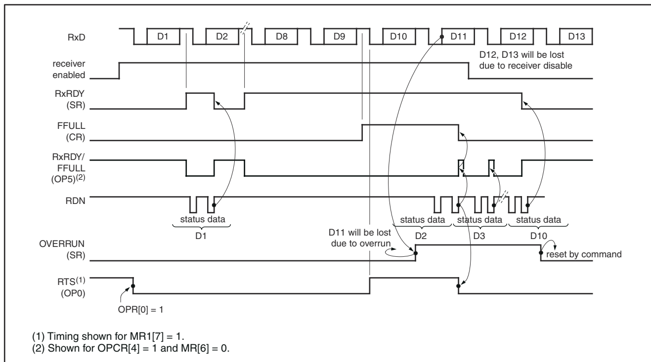
图 4-13. Receiver Timing
