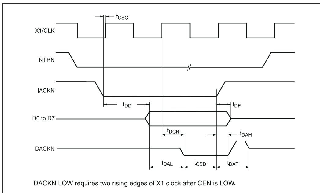
图 4-6. Interrupt Cycle Timing (68xxx Mode)
