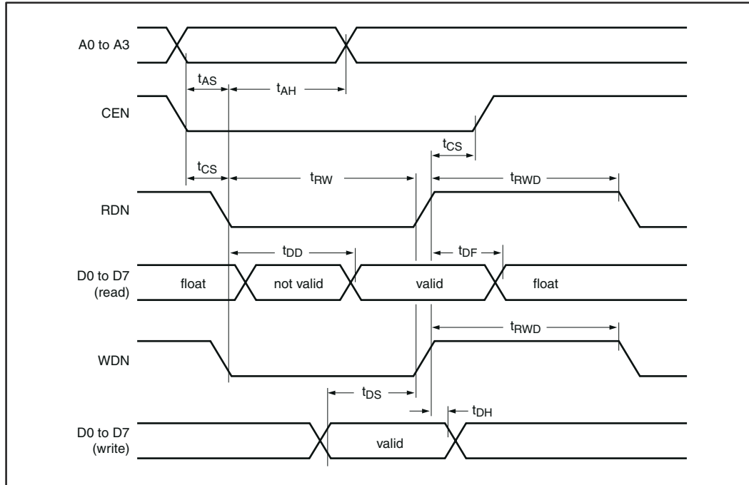
图 4-3. Bus Timing (80xxx Mode)
