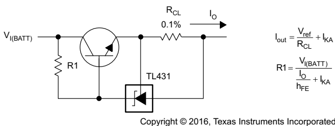
Figure 37. Voltage Monitor
