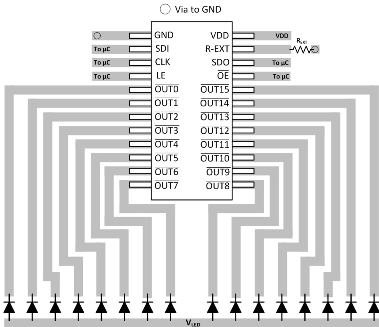
图 11-1. Layout Recommendation
