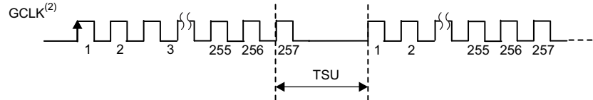
Figure 19. Timing Diagrams
