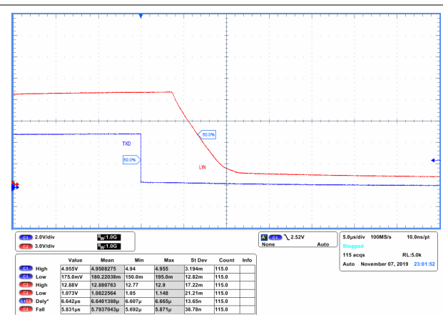
图 10-3. Recessive to Dominant Propagation Delay
