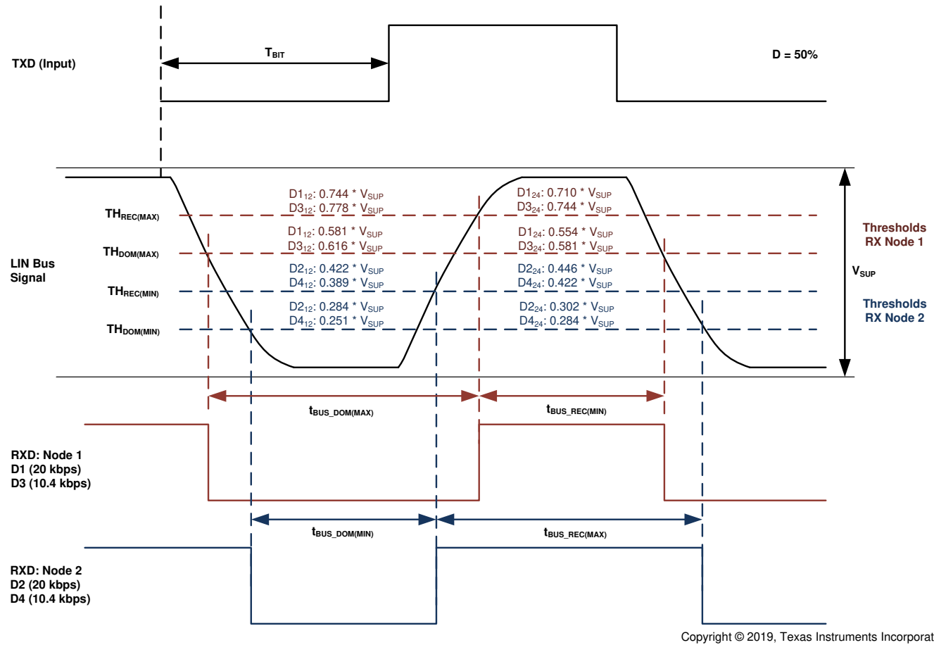
图 8-12. Definition of Bus Timing Parameters
