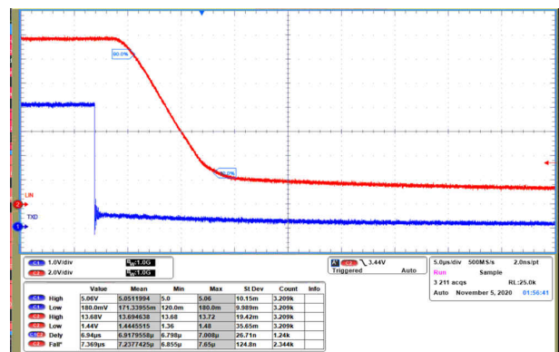
图 10-3. Recessive to Dominant Propagation Delay
