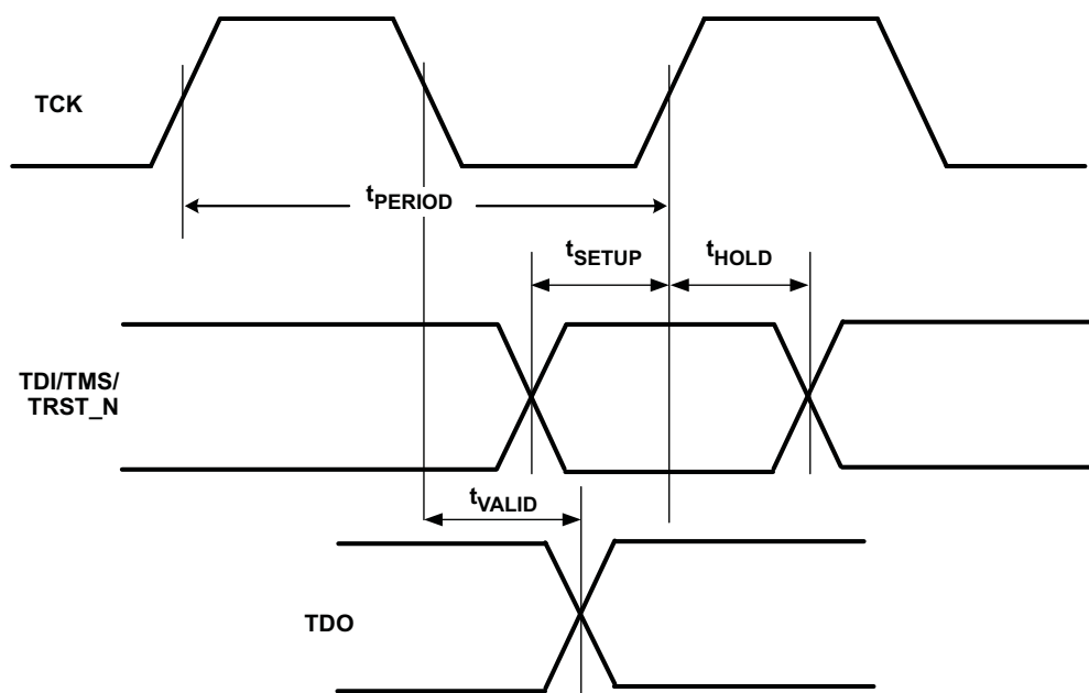
Figure 4-14. JTAG Timing
