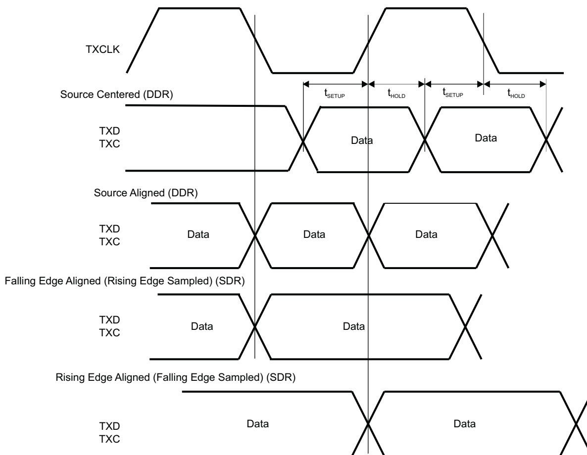
Figure 2-18. Transmit Interface Timing
