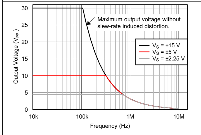
图 23. Maximum Output Voltage vs Frequency
