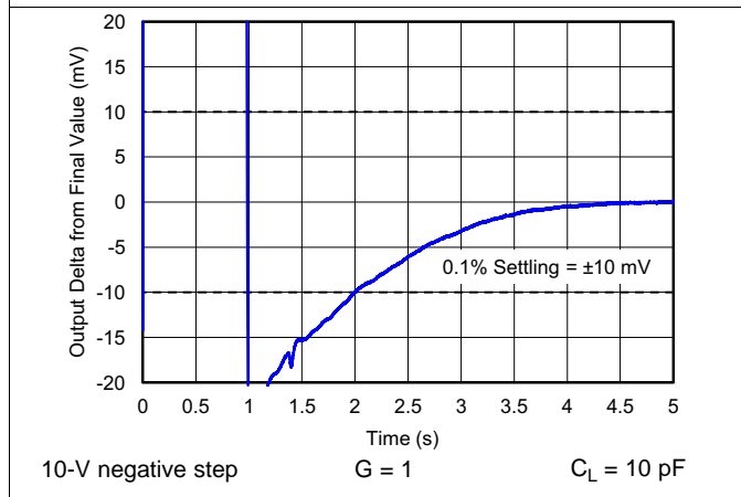
图 19. Large-Signal Step Response
