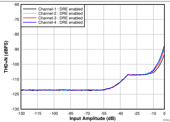
图 7. THD+N vs Input Amplitude With DRE Enabled
