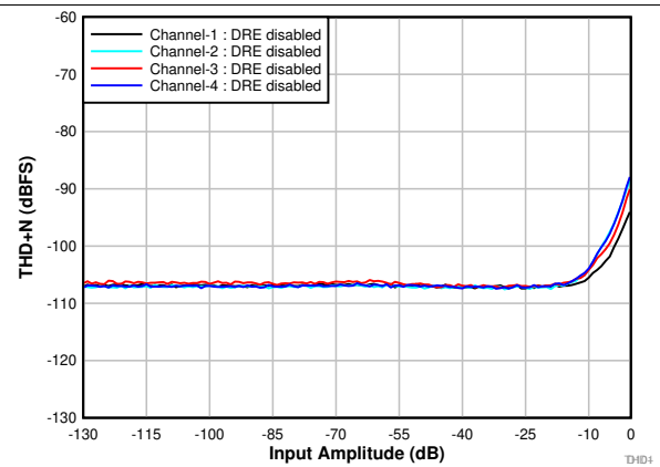
图 8. THD+N vs Input Amplitude With DRE Disabled
