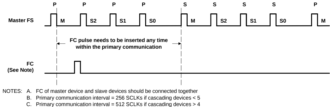
Figure 3–6. Output When Hardware Secondary Serial Communication Is Requested (Three Slaves)
