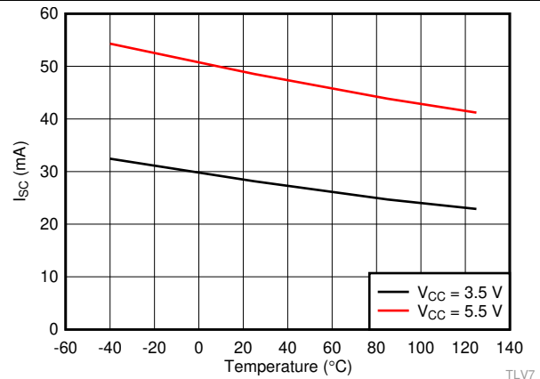
V_{CM} = V_{CC}/2
