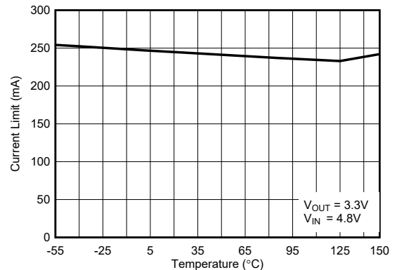
图 6-18. Current Limit vs Junction Temperature for New Chip
