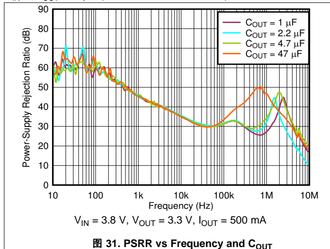
图 31. PSRR vs Frequency and C_{OUT}
