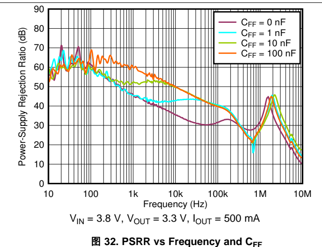
图 32. PSRR vs Frequency and C_{FF}
