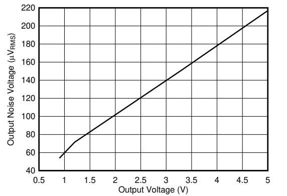
I_{OUT} = 500\text{mA} , C_{OUT} = 1\mu\text{F} , V_{RMS} \text{ BW} = 10\text{Hz to } 100\text{kHz} 图 5-6. Output Noise Voltage vs V_{OUT}
