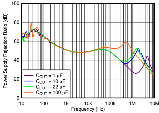
V_{IN} = 4.3\text{V} , V_{OUT} = 3.3\text{V} , I_{OUT} = 500\text{mA} 图 5-3. PSRR vs Frequency and C_{OUT}
