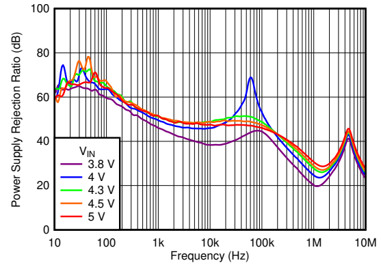
V_{OUT} = 3.3\text{V} , C_{OUT} = 1\mu\text{F} , I_{OUT} = 500\text{mA} 图 5-2. PSRR vs Frequency and V_{IN}
