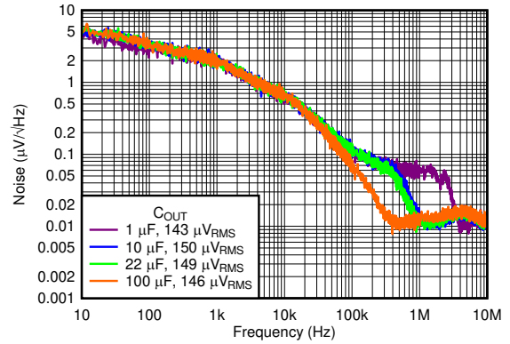
V_{OUT} = 3.3\text{V} , V_{RMS} \text{ BW} = 10\text{Hz to } 100\text{kHz} 图 5-4. Output Spectral Noise Density vs Frequency and C_{OUT}
