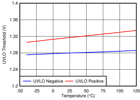
图 5-25. UVLO Threshold vs Temperature
