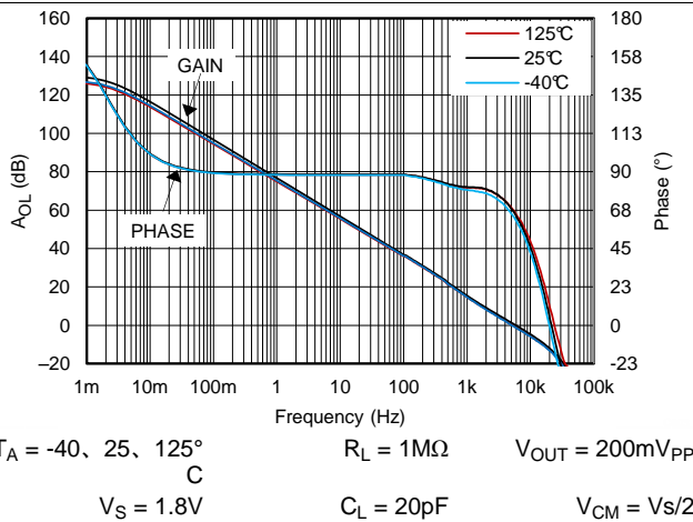
Figure 33. 开环增益和相位, 1.8V, 1MΩ 负载
