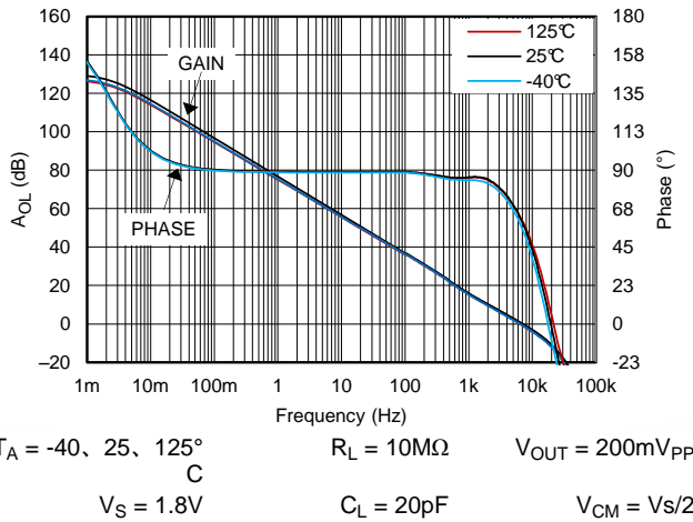
Figure 31. 开环增益和相位, 1.8V, 10MΩ 负载
