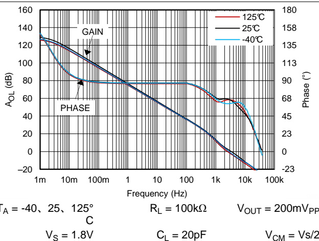
Figure 35. 开环增益和相位, 1.8V, 100kΩ 负载
