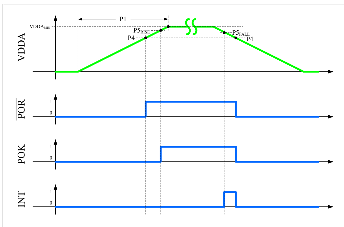
图 24-4. Power Assertions versus VDDA Levels
