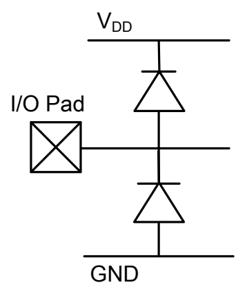
图 24-17. ESD Protection on Non-Fail-Safe Pins
