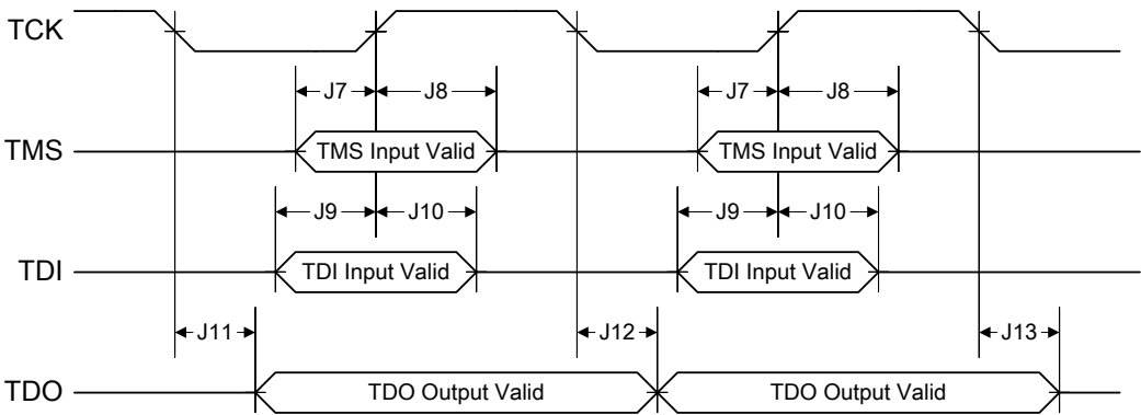
图 24-3. JTAG Test Access Port (TAP) Timing
