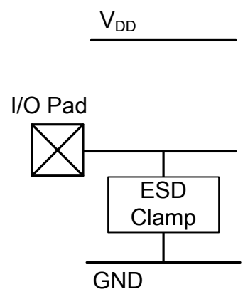
图 24-16. ESD Protection on Fail-Safe Pins
