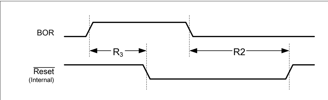
图 22-10. Brown-Out Reset Timing
