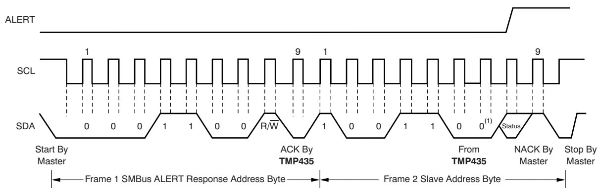
Figure 18. Two-Wire Timing Diagram for Two-Byte Read Format
