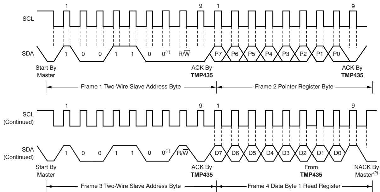
Figure 16. Two-Wire Timing Diagram for Write Word Format
