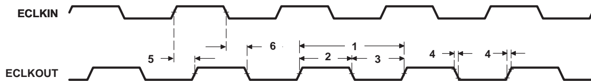
Figure 35. ECLKOUT Timings
