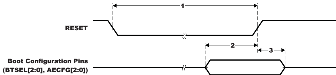
Figure 7-4. Reset Timing
