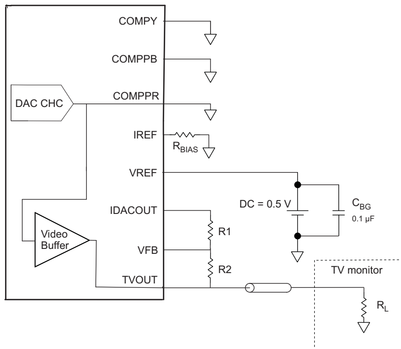
Figure 7-40. SD Video Buffer Application Example
