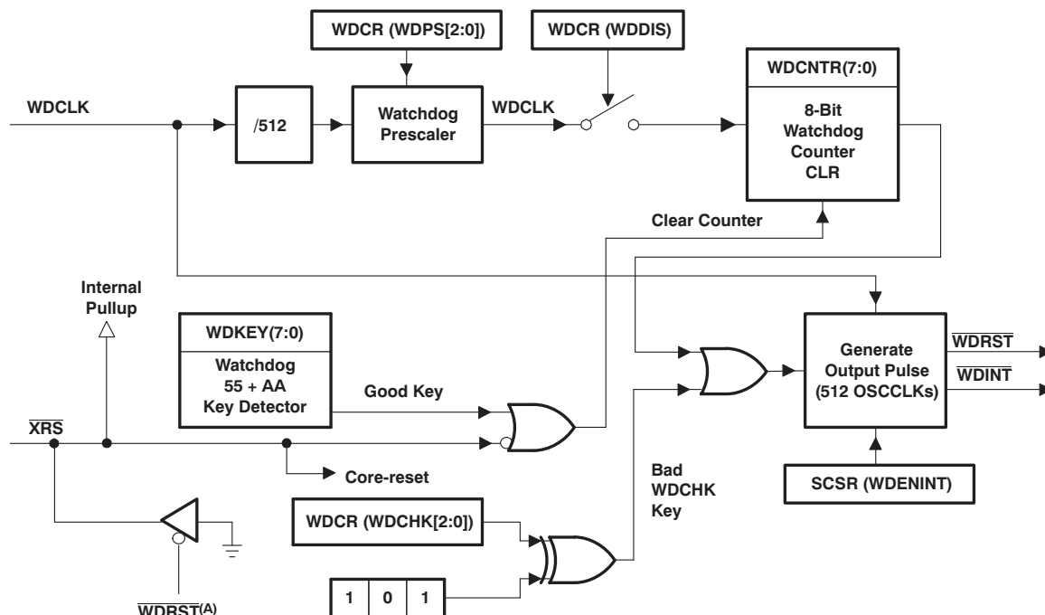
Figure 2-10. CPU-watchdog Module
