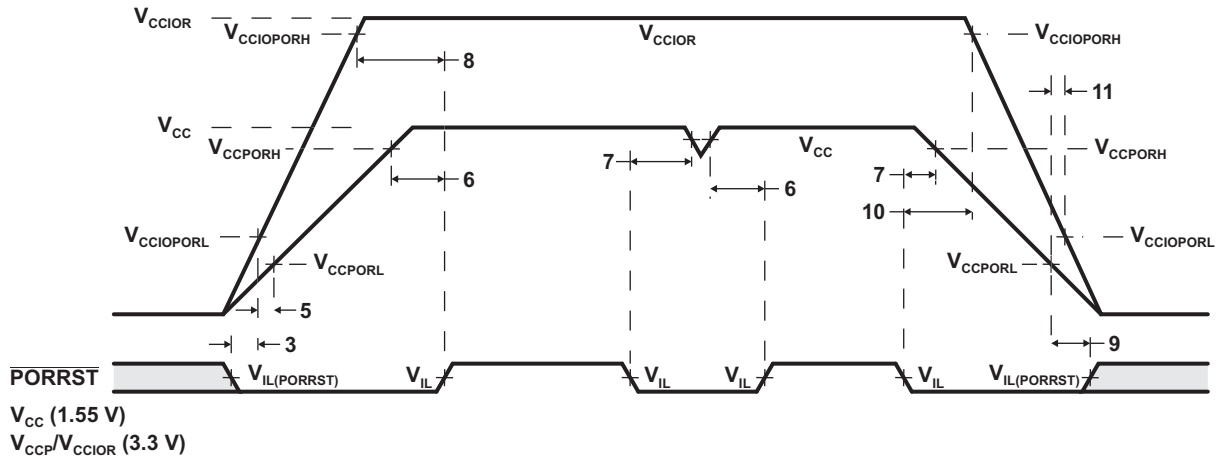
Figure 5-1. \overline{\text{PORRST}} Timing Diagram
