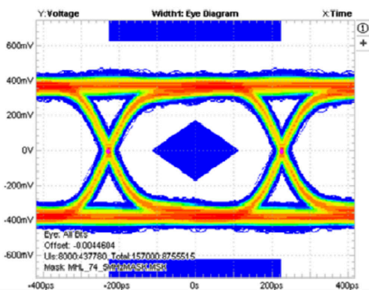
图 9-6. Eye Pattern: 2.2 Gbps with No Device
