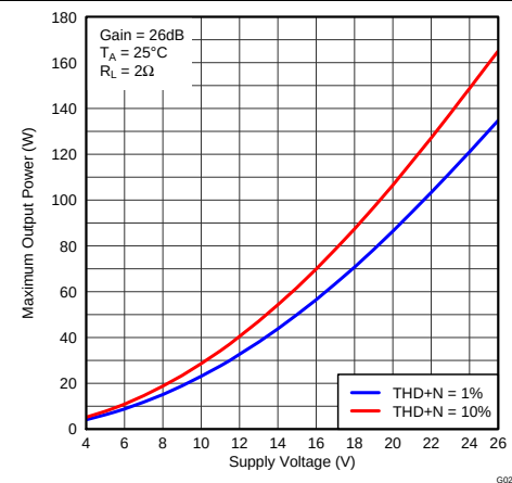
图 22. Maximum Output Power (PBTL) vs Supply Voltage
