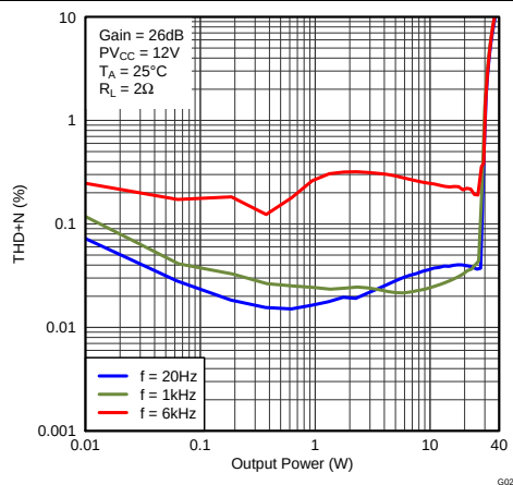
图 21. Total Harmonic Distortion + Noise (PBTL) vs Output Power
