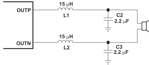
图 8-5. Typical LC Output Filter, Cutoff Frequency of 27 kHz, Speaker Impedance = 6 Ω
