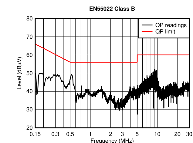
图 8-8. Conducted Emission - Line
