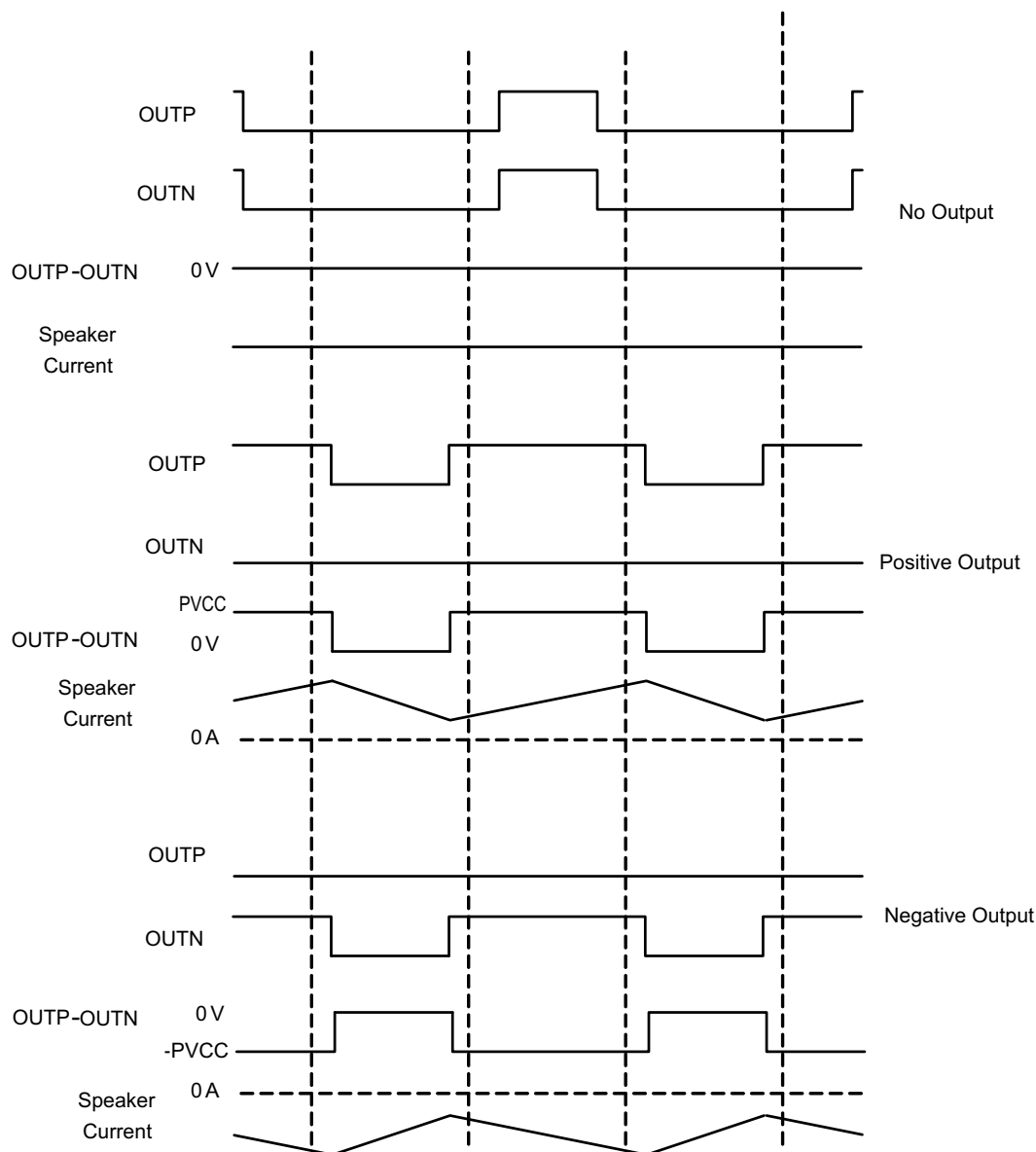
图 7-3. Low-Idle-Current 1SPW Modulation
