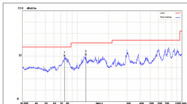
图 8-6. Radiated Emission - Horizontal
