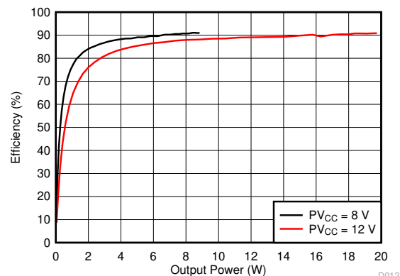
图 6-8. Efficiency vs Output Power (BTL)
