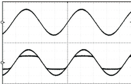
图 7-1. PLIMIT Circuit Operation
