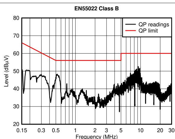
图 8-9. Conducted Emission - Neutral
