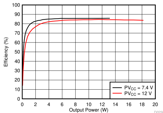
图 6-20. Efficiency vs Output Power, 4 \Omega
