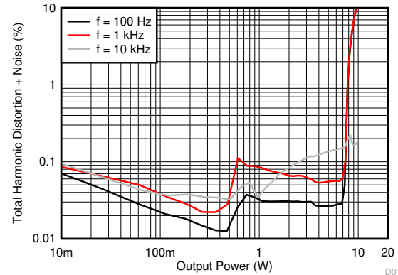
A. AVCC=PVCC = 12 V, 1 W Load = 8 Ω 1SPW
