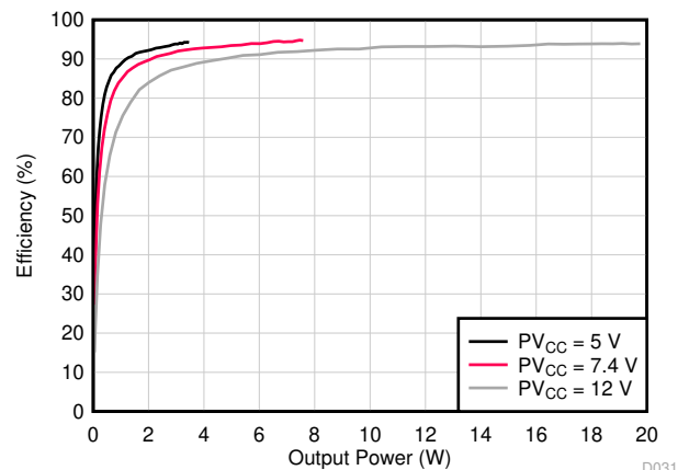
图 6-31. Efficiency vs Output Power, 4 Ω
