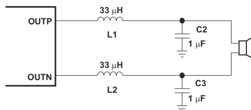
图 8-4. Typical LC Output Filter, Cutoff Frequency of 27 kHz, Speaker Impedance = 8 Ω
