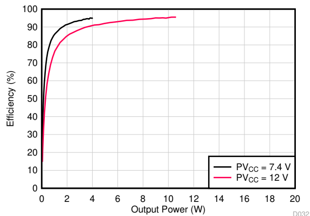
图 6-30. Efficiency vs Output Power, 8 Ω
