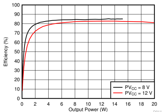
图 6-7. Efficiency vs Output Power (BTL)
