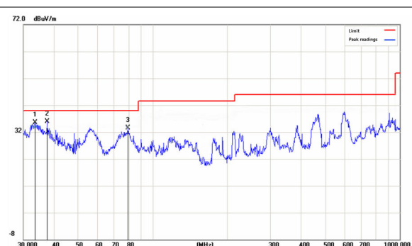
图 8-7. Radiated Emission - Vertical
