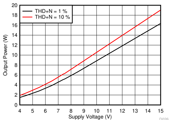
图 6-19. Output Power vs Supply Voltage, 4 \Omega
