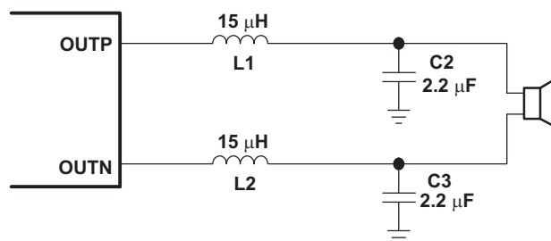
Figure 28. Typical LC Output Filter, Cutoff Frequency of 27 kHz, Speaker Impedance = 6 Ω
