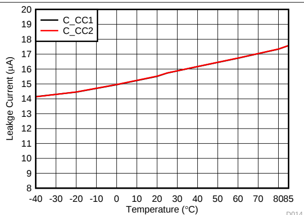
图 19. C_CC Path Leakage Current vs Ambient Temperature at C_CC = 5.5 V
