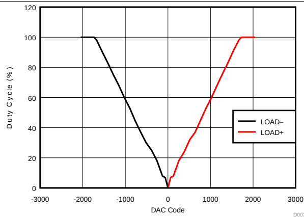
Figure 60. DAC Code vs Duty Cycle for LOAD Outputs
