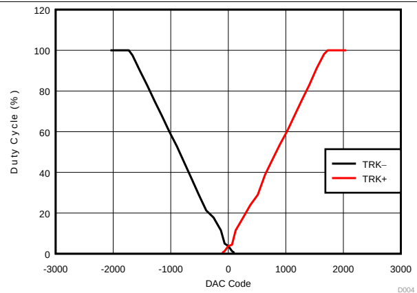
Figure 61. DAC Code vs Duty Cycle for TRK Outputs
