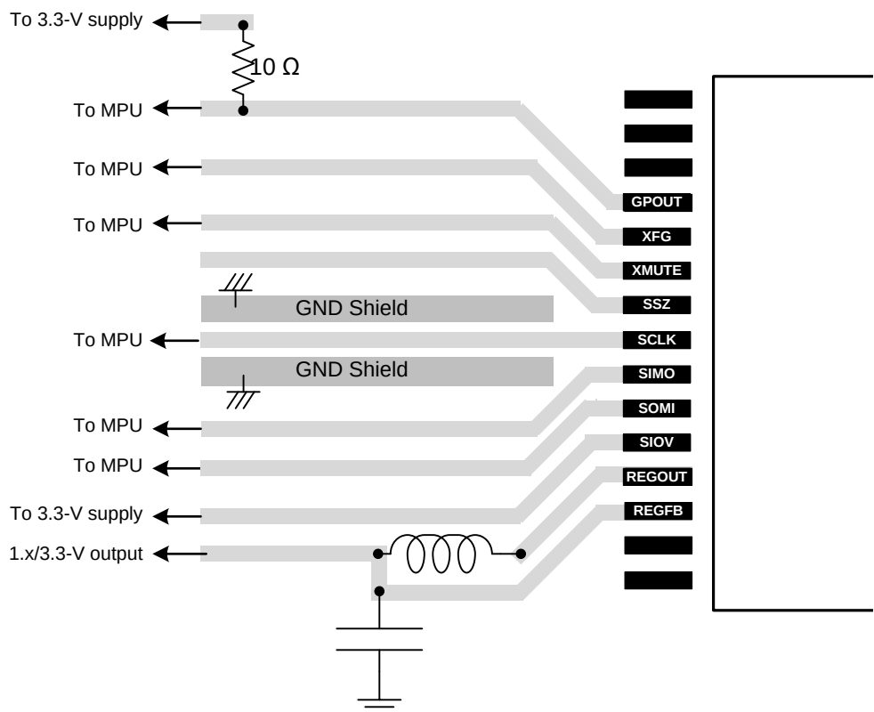
Figure 62. Layout Recommendation
