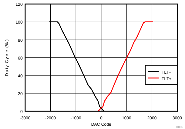
Figure 4. DAC Code vs Duty Cycle for TLT Outputs
