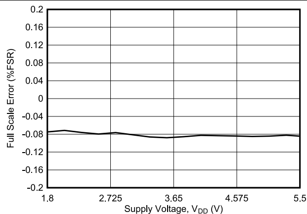
图 6-27. Full-Scale Error vs Supply Voltage
