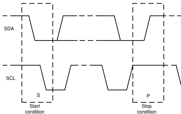
图 7-3. Start and Stop Conditions
