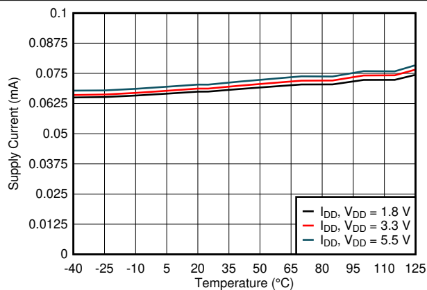
图 6-33. Power-Down Current vs Temperature
