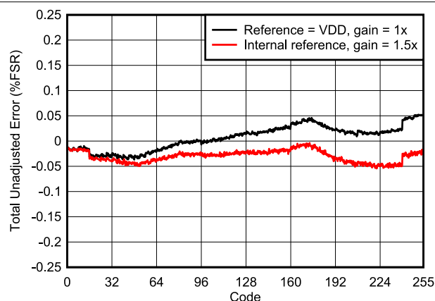
图 6-3. Total Unadjusted Error vs Digital Input Code
