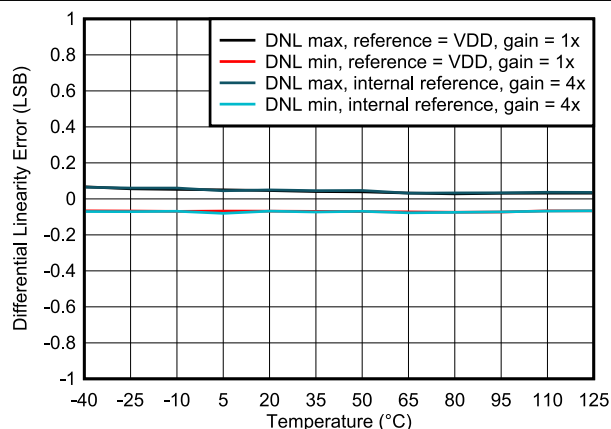
图 6-15. Differential Linearity Error vs Temperature
