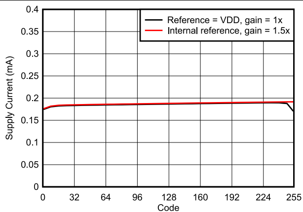
图 6-28. Supply Current vs Digital Input Code
