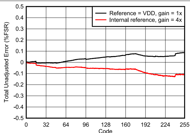
图 6-13. Total Unadjusted Error vs Digital Input Code
