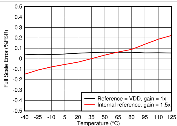
图 6-10. Full-Scale Error vs Temperature
