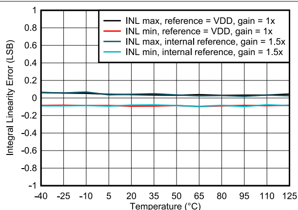
图 6-4. Integral Linearity Error vs Temperature
