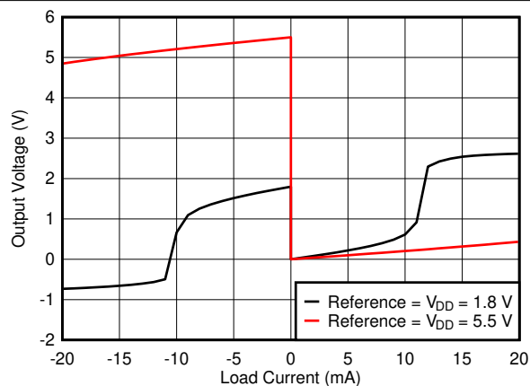
图 6-34. Source and Sink Capability
