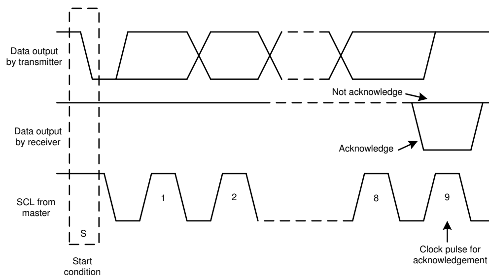
图 7-2. Acknowledge and Not Acknowledge on the I 2 C Bus
