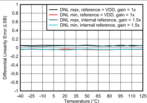
图 6-5. Differential Linearity Error vs Temperature
