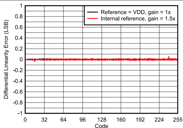
图 6-2. Differential Linearity Error vs Digital Input Code
