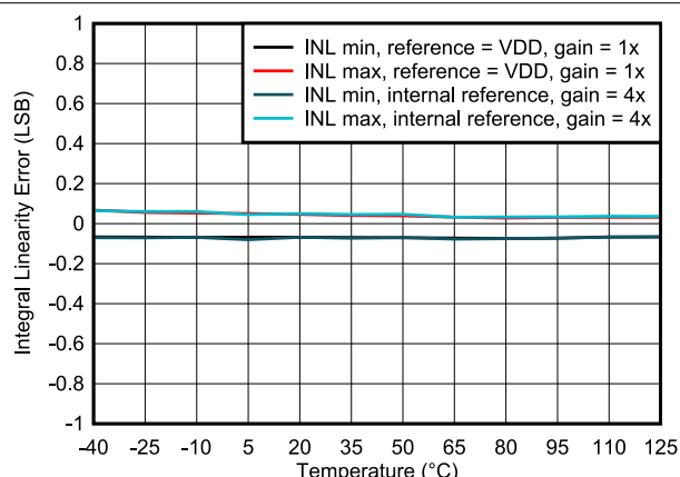
图 6-14. Integral Linearity Error vs Temperature
