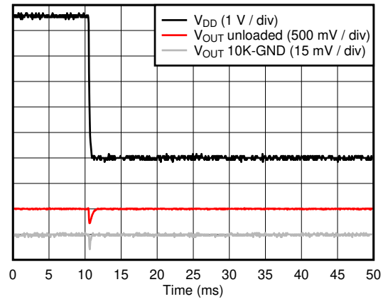
图 6-40. Power-off Glitch
