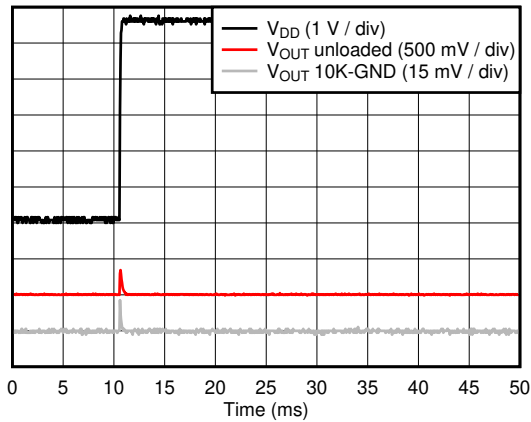
图 6-39. Power-on Glitch
