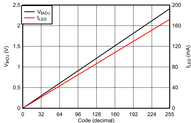
图 8-2. Digipot Code vs LED Current
