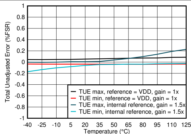
图 6-6. Total Unadjusted Error vs Temperature
