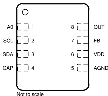
图 5-1. DSG Package, 8-Pin WSON, Top View
