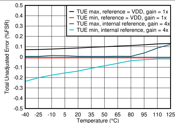
图 6-16. Total Unadjusted Error vs Temperature
