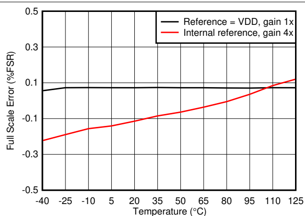
图 6-20. Full-Scale Error vs Temperature
