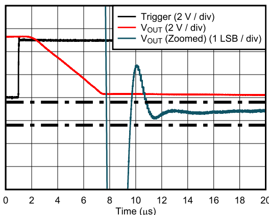
图 6-36. Glitch Impulse, Falling Edge, 1-LSB Step
