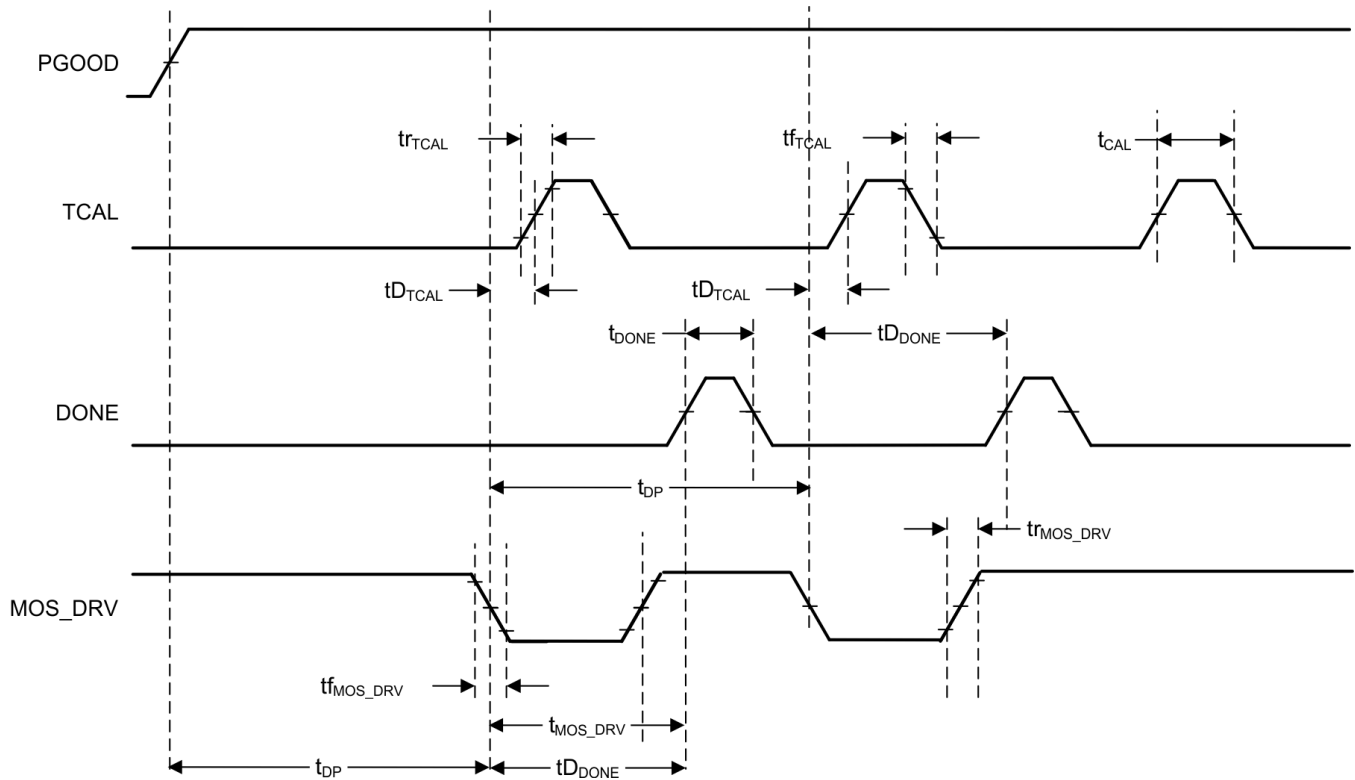
Figure 1. Timing Diagram
