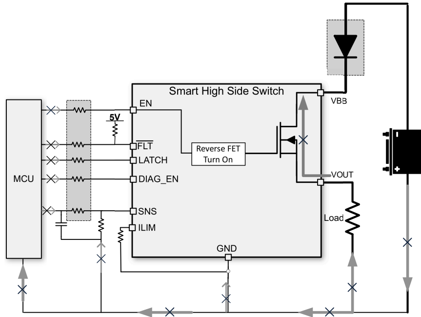
图 7-20. Reverse Protection With Block Diode
