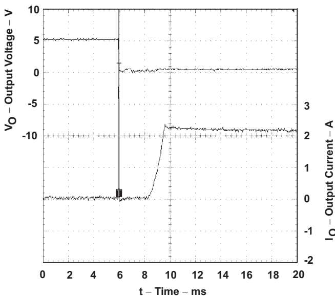
Figure 4. TPS2015 Short-Circuit Current. Short is Applied to Enabled Device, V_{I(IN)} = 5 V
