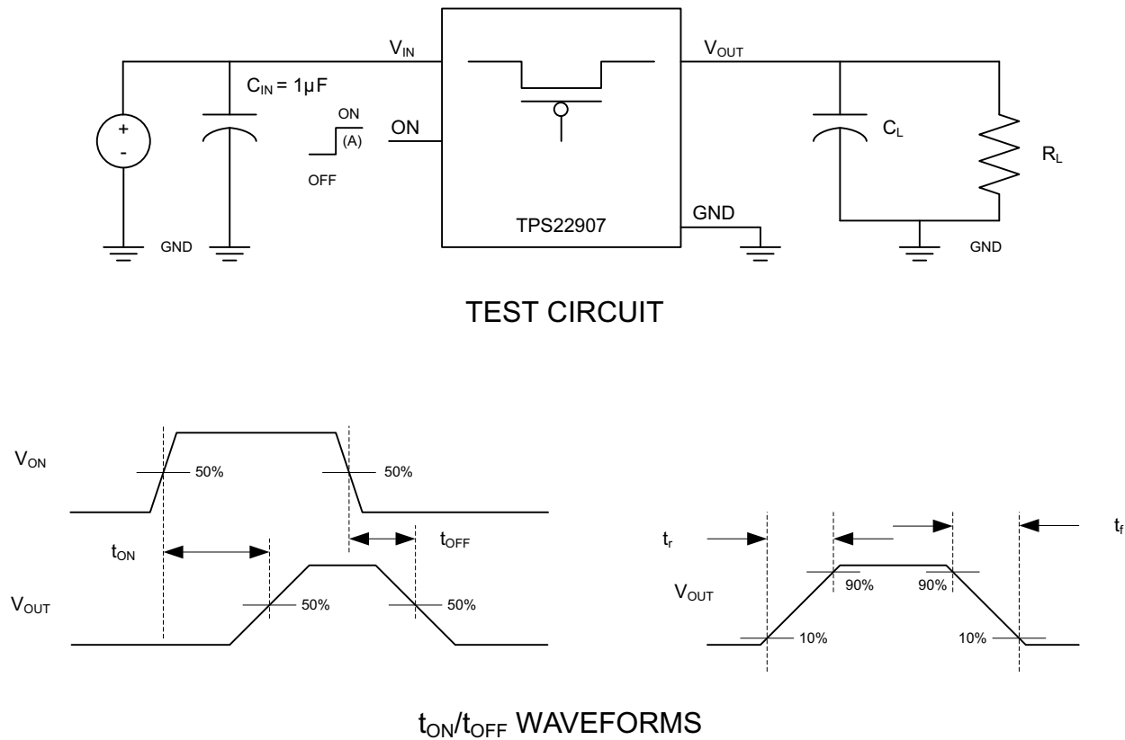
Figure 22. Test Circuit and t_{ON}/t_{OFF} Waveforms
