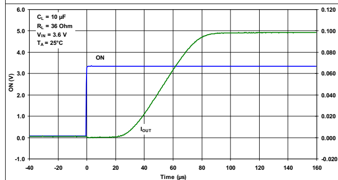
Figure 21. t_{ON} Response
