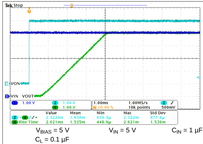
Figure 34. t_R at V_{BIAS} = 5\text{ V}
