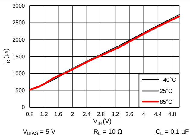
Figure 28. t_R vs V_{IN}
