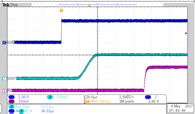
图 20. Low Inrush Current at 0.65 V IN
