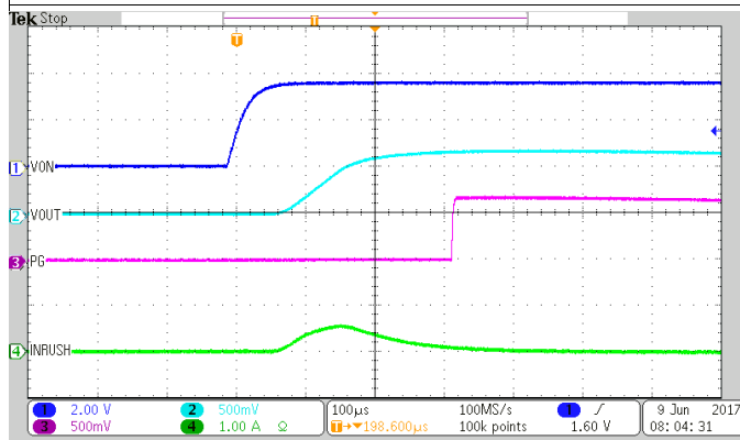
图 19. High Inrush Current at 3.6 V IN
