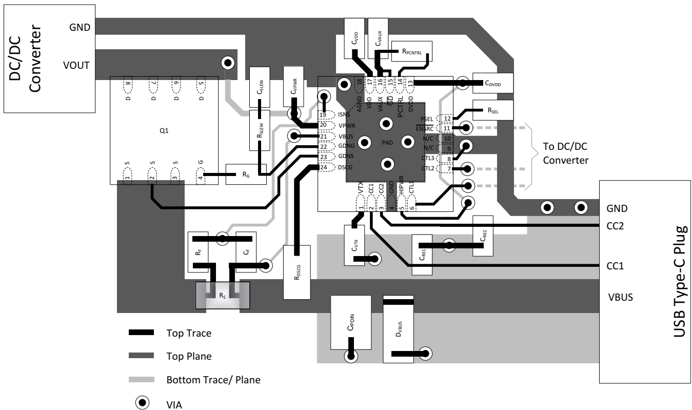
Figure 72. Example Layout
