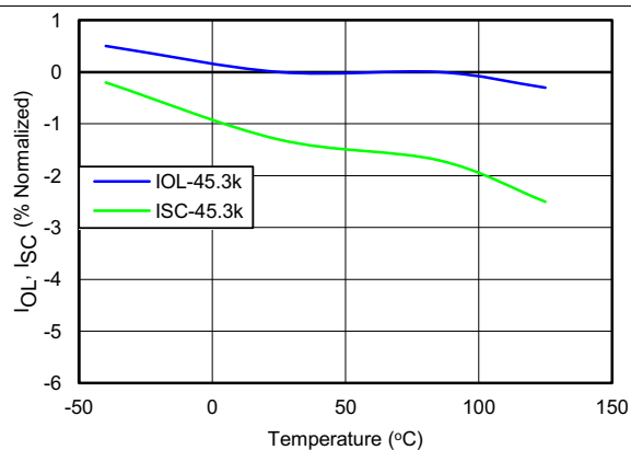
Figure 14. I_{OL} , I_{SC} vs Temperature
