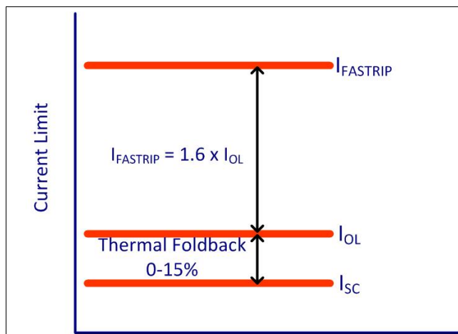
Figure 37. Fast-Trip Current
