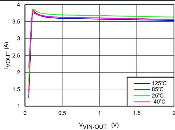
Figure 13. I_{OUT} vs V_{VIN-OUT}
