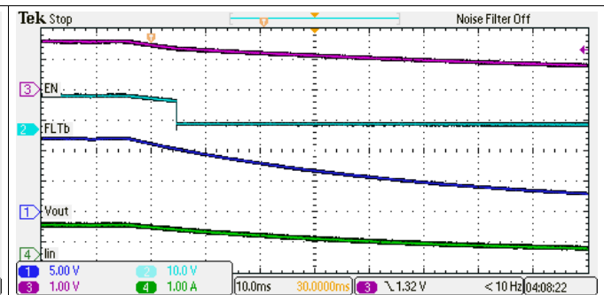
Figure 45. Hold-up Power When VIN Fails
