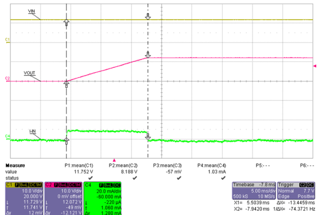
Figure 18. TRANSIENT: OUTPUT RAMP ( C_{dVdT} = 1\text{ nF} ): TPS2592Ax
