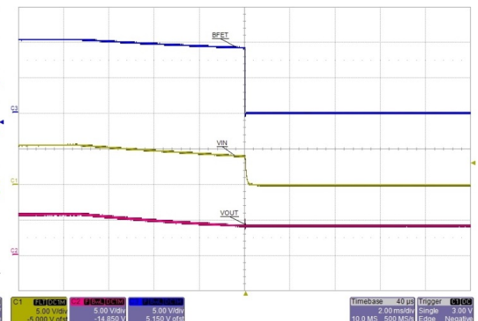
Figure 24. TRANSIENT: TURN OFF DELAY TO BFET ( \text{VIN}\downarrow )
