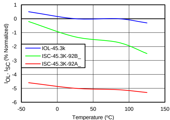
Figure 32. I_{OL} , I_{SC} vs TEMPERATURE (45.3kΩ)
