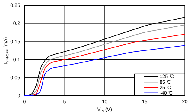
Figure 2. I_{\text{VIN-OFF}} vs V_{\text{IN}} ACROSS TEMPERATURE
