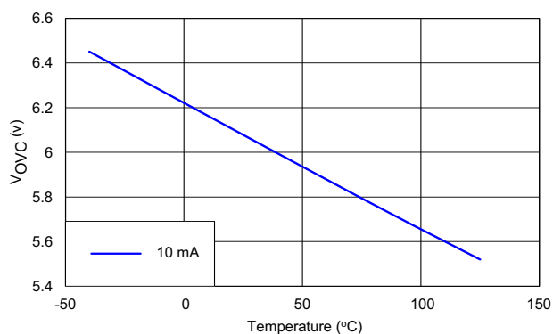
Figure 6. V_{\text{OVC}} vs TEMPERATURE (TPS2592Bx)
