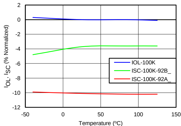
Figure 31. I_{OL} , I_{SC} vs TEMPERATURE (100kΩ)
