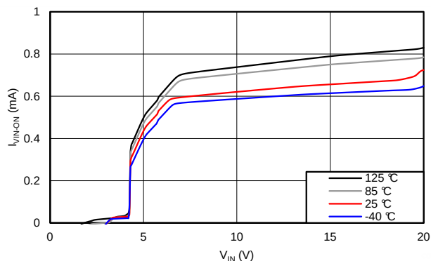
Figure 4. I_{\text{VIN-ON}} vs V_{\text{IN}} ACROSS TEMPERATURE (TPS2592Bx)
