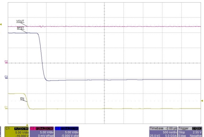
Figure 22. TURN OFF DELAY TO BFET ( \text{EN}\downarrow )
